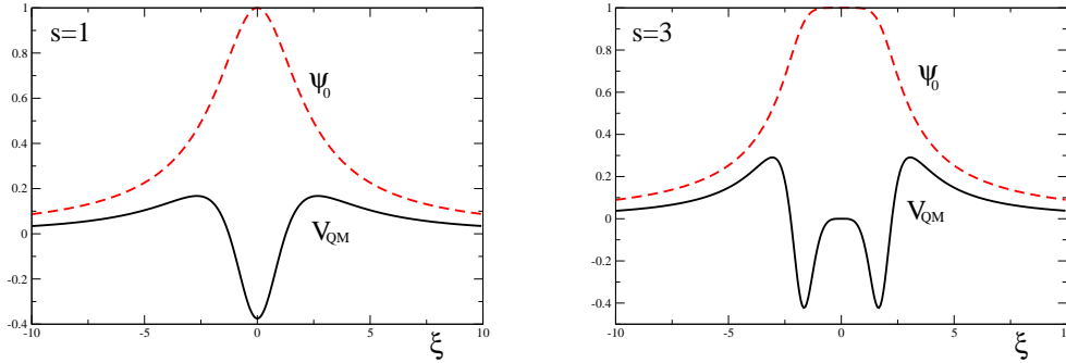
FIG. 2: V_{QM} and the zero mass mode for walls with s = 1 and s = 3 .
