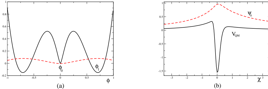
FIG. 3: Figure (a) shows the scalar field potential (continuous line) and superpotential (dashed line) for the asymmetric brane (30-34), with \beta > \alpha > 0 . Figure (b) gives V_{QM} and the (arbitrarily normalized) zero mode for the same values of the parameters.
