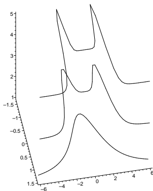
FIG. 1: Energy density as a function of \xi for double walls with s = 1, 3, 5 .
