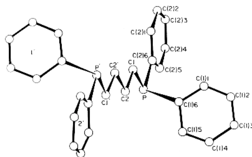
Fig. 1. Perspective view of the molecule showing atom numbering.
